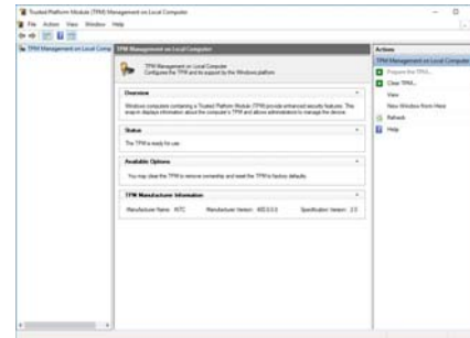
Figure 27 Trusted Plat- form Module (TPM) Manage- ment on Local Computer Ad- ministration
